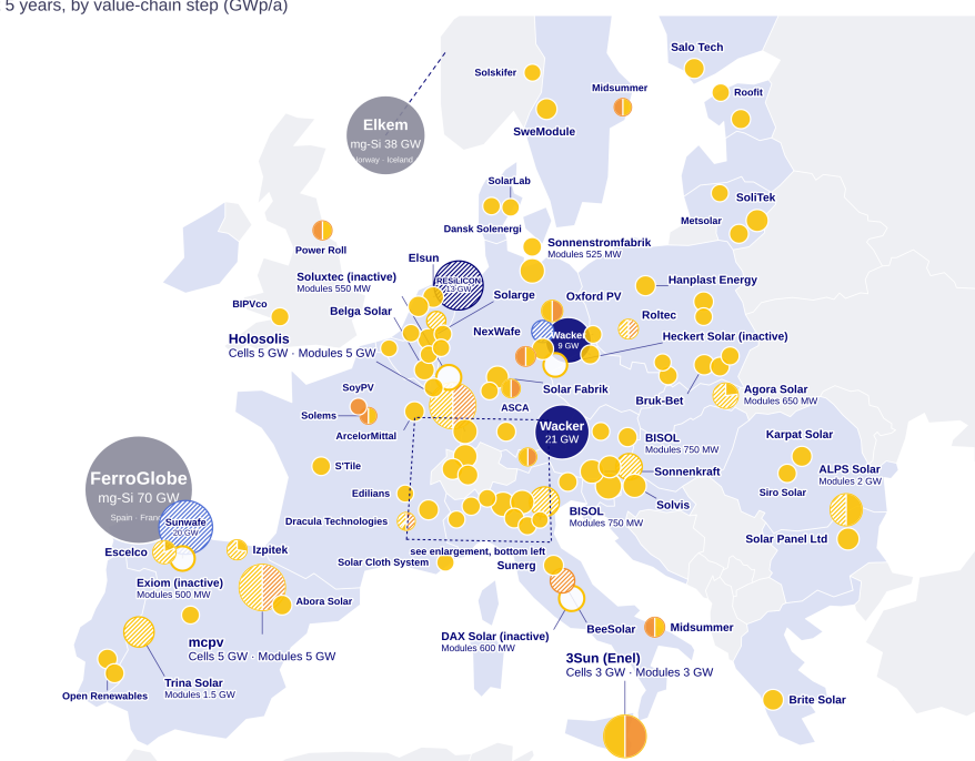
Figure 3 | Solar PV manufacturing in Europe – potential annual production capacity in the next five years, by value-chain step and site. Source: Becquerel Institute (2026); ESMC survey of European module producers (2025); Fraunhofer ISE / SolarPower Europe (Sept. 2025), updated by ESMC (Sept. 2026).
