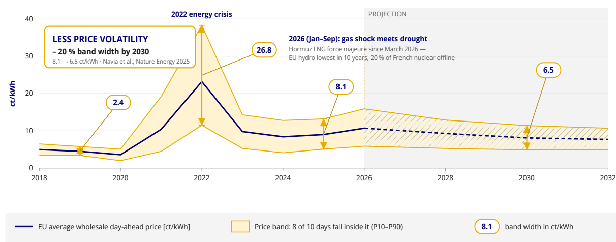
Figure 4 | EU wholesale power price and volatility, 2018–2032 – the 2022 shock, and the narrowing band that solar delivers. Source: Ember / ENTSO-E day-ahead prices; volatility outlook Navia et al., Nature Energy 10, 329 (2025).
