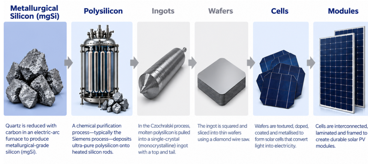
Figure 1 | Europe has production capacities mainly at the start and end of the supply chain. However, the crucial ingot and wafer stage is missing.
